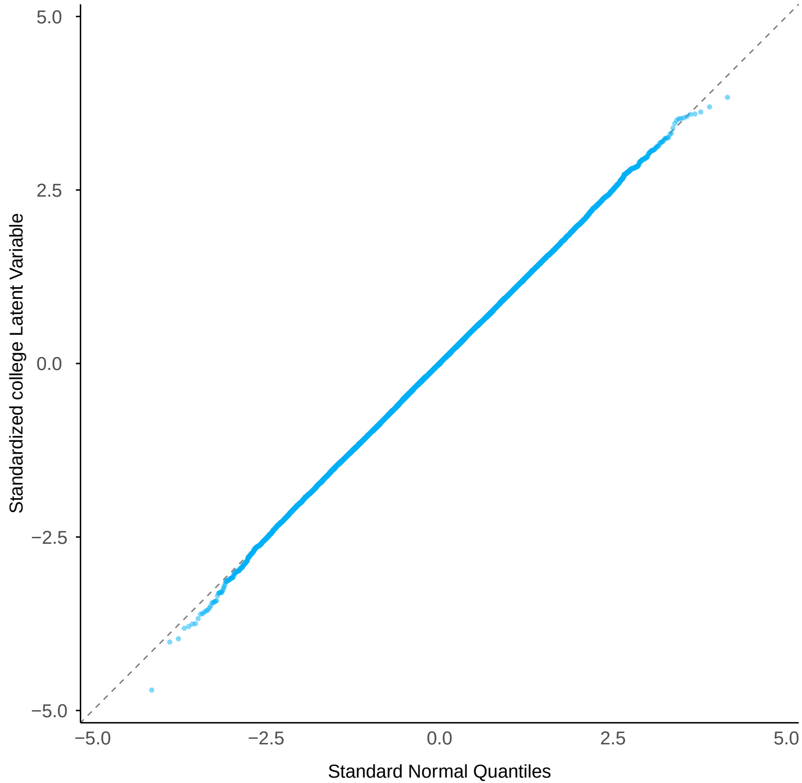
Normal Q-Q: college Latent Variable
